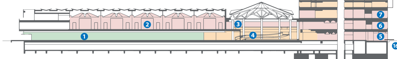
断面図 Cross-sectional View
